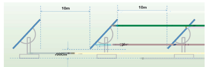
Figure 1. Fixed axis
